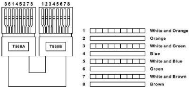
Cross interconnection method
